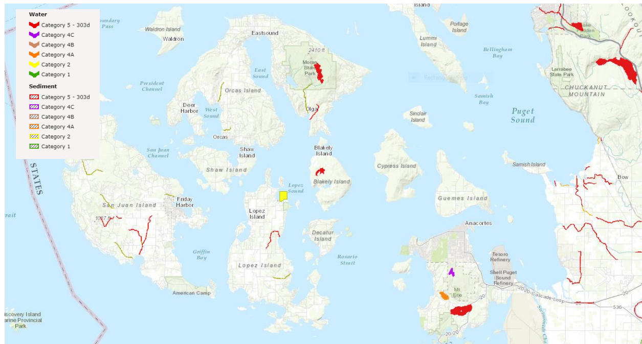
Figure 27: Freshwater or sediments that either have been identified as a “Water of Concern” (Category 2) or a “Polluted Water” (Category 4 and 5).
