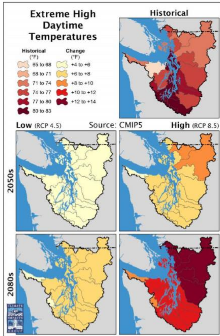
Figure 9: Changes in Extreme High Daytime Temperature for Low RCP (4.5) and High RCP (8.5) IPCC emissions scenarios. Figure source: Mauger et al., 2015. Figure created by Robert Norheim, CIG, based on the CMIP5 projections used in the IPCC 2013 report. Data source: Mote et al 2015.
